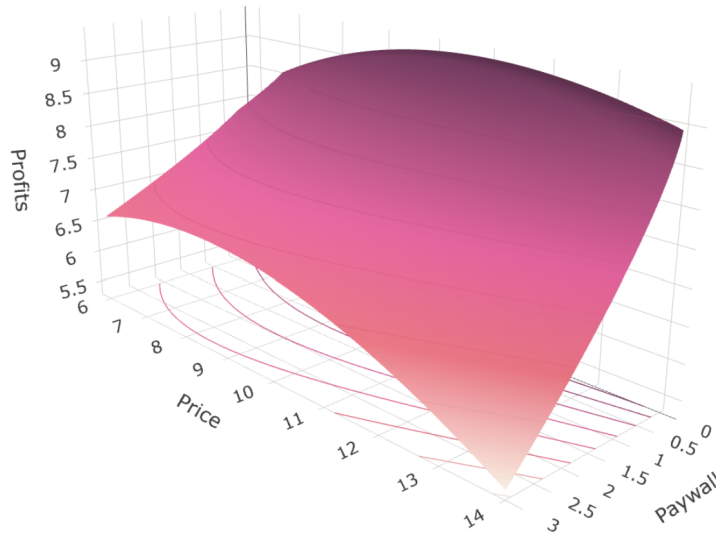
Figure 8: Profit over \bar{x} and p
